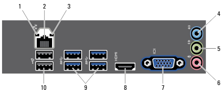
Figur 2. Bakpanelsvy
